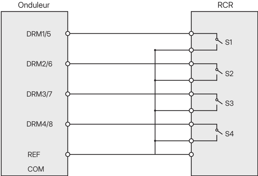
Figure 7-5 Connexion RCR
